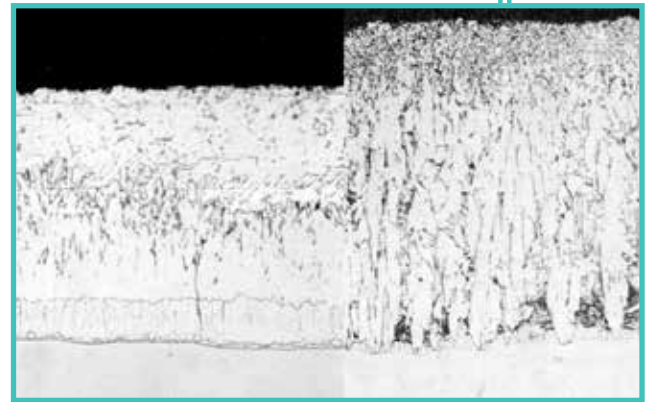
FIGURE 7: RECOMMENDED SILICON VS. REACTIVE STEEL
