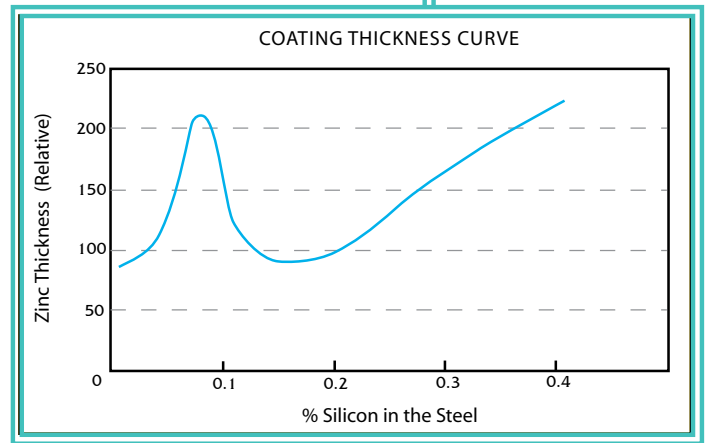
FIGURE 6: SANDELIN CURVE
