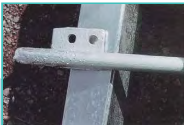
FIGURE 35: WELDING SPATTER (REJECTABLE)
