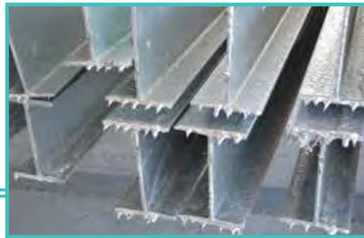
FIGURE 18: DRAINAGE SPIKES (ACCEPTABLE AFTER REMOVAL OR FILING)
