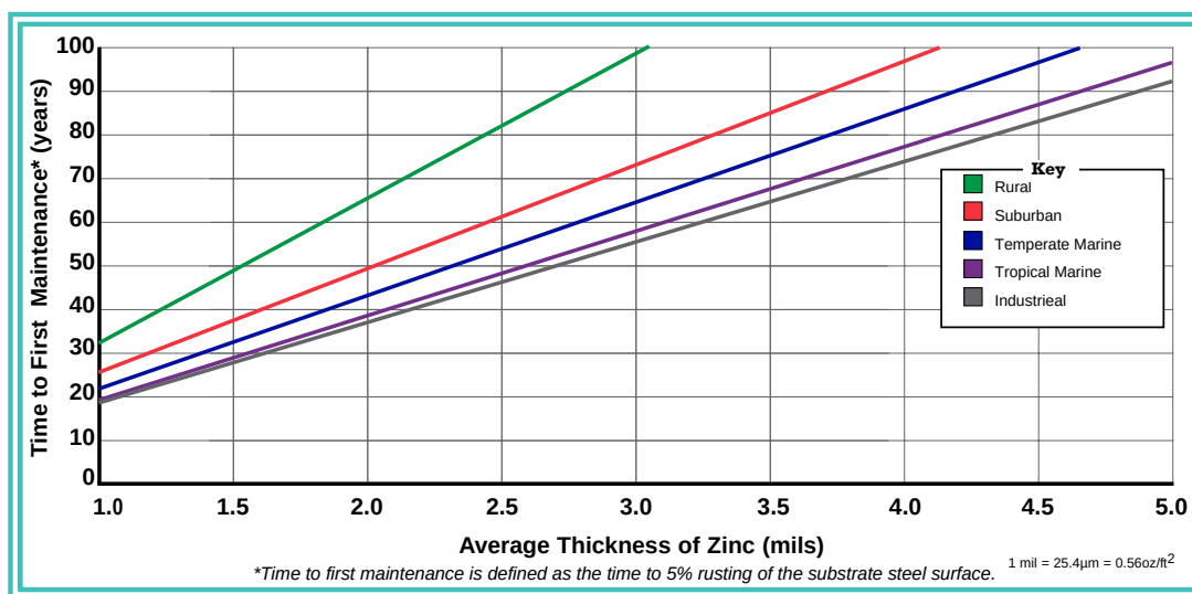
FIGURE 1: TIME TO FIRST MAINTENANCE OF HOT-DIP GALVANIZED COATINGS
