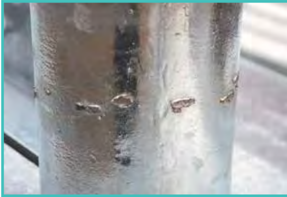
FIGURE 14: CHAIN AND WIRE MARKS (ACCEPTABLE UNLESS BARE STEEL IS EXPOSED)
