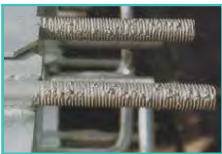
FIGURE 15B: CLOGGED THREADS (ACCEPTABLE AFTER THREADS ARE CLEANED)
