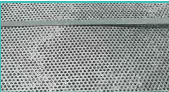
FIGURE 15A: CLOGGED HOLES < 1/2 IN (ACCEPTABLE), HOLE SIZE ≥ 1/2 IN (ACCEPTABLE AFTER CLEANING)
